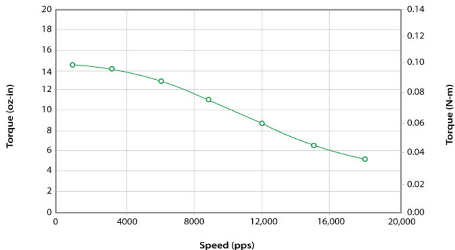
3709V-03 24VDC, 1.2 Amps/Phase, Bipolar, 1/2 Stepping
