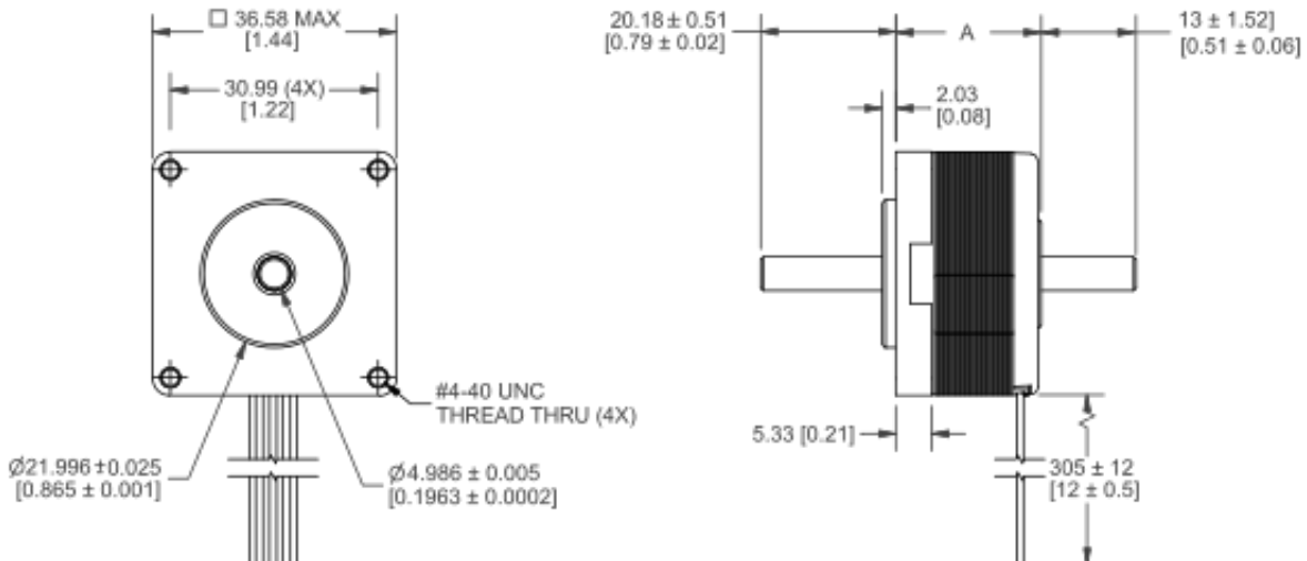
3709V-03 24VDC, 1.2 Amps/Phase, Bipolar, 1/2 Stepping
